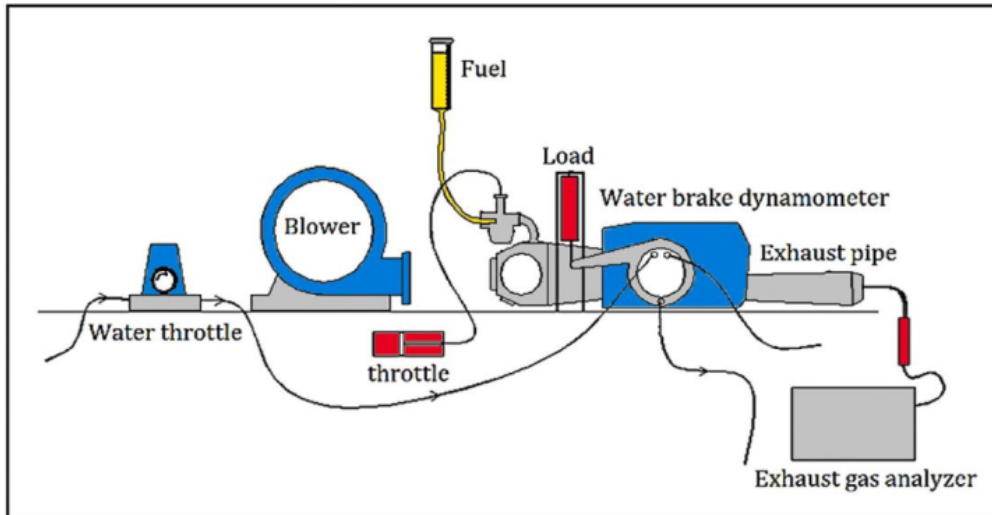
Fig. 2. The research apparatus.
