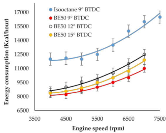
Fig. 7. Energy consumption of SI engine at various ignition timings.
