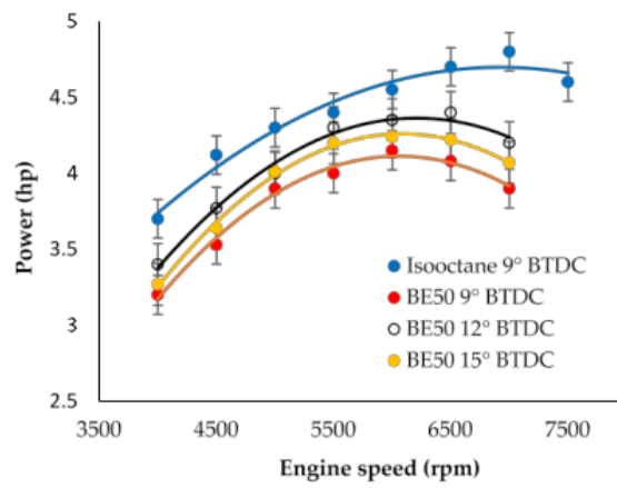
Fig. 4. Engine power at various ignition timings.
