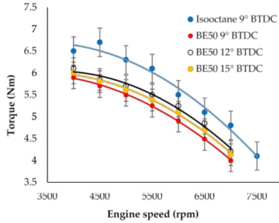
Fig. 3. Engine torque at various ignition timings.
